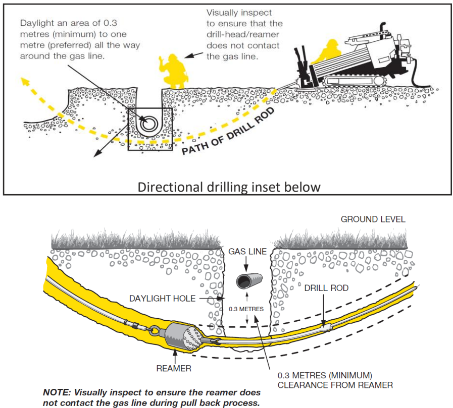
Figure 1: Observing and maintaining safe clearances when boring
